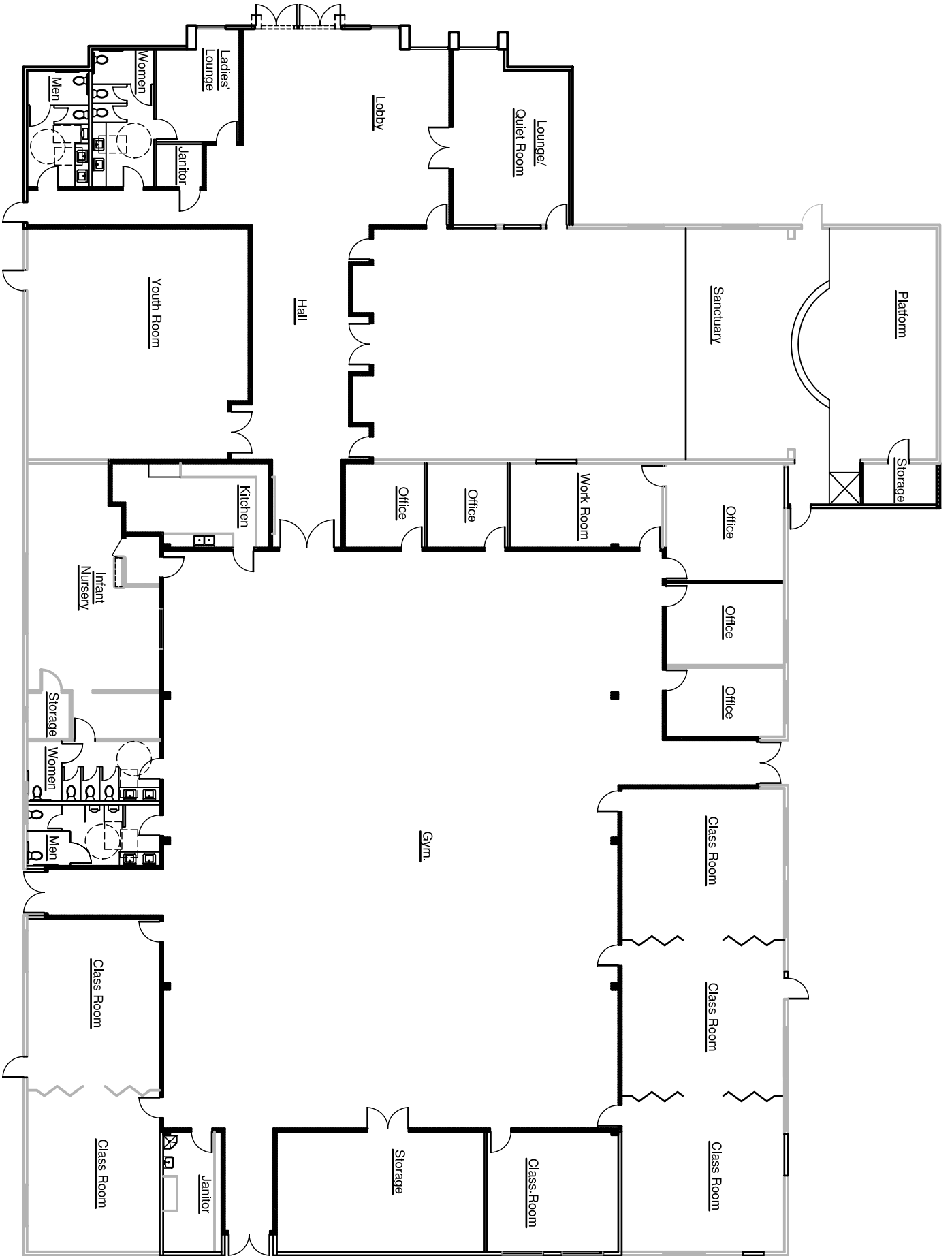
FLOOR & DIMENSION PLAN SCALE: 1/8" = 1'-0"
